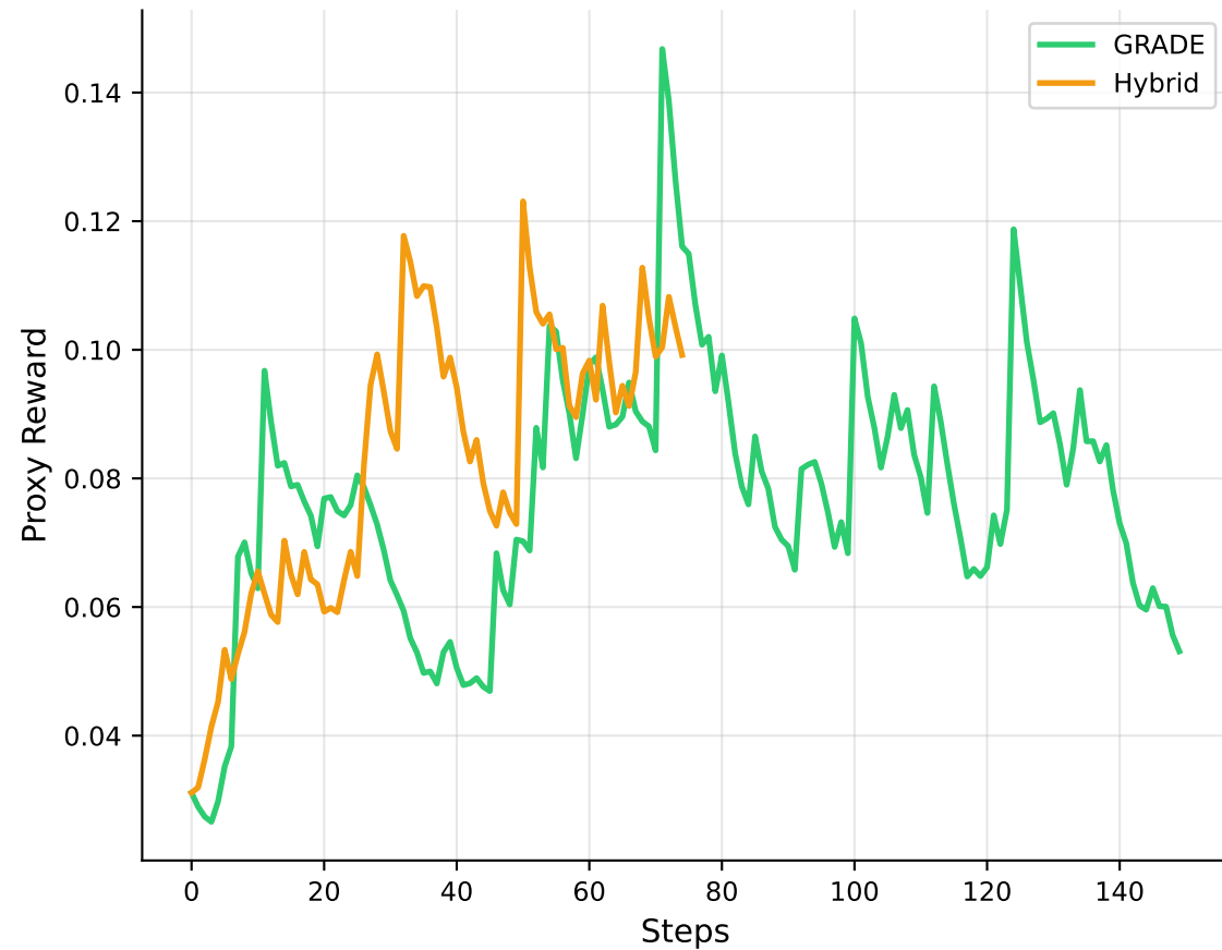
(a) Proxy Reward
